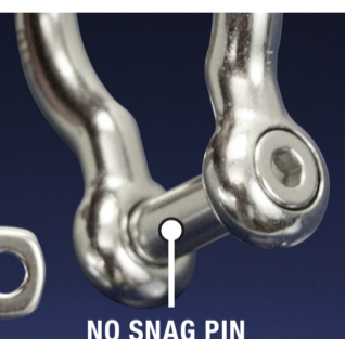
Pin head sits flush with sides of shackle body to prevent snagging.
