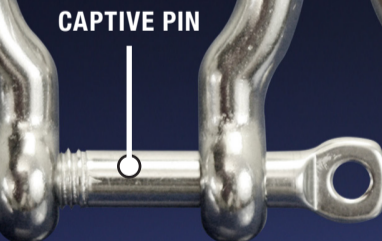
Design allows pin to open and install attachments, but keeps pin from being fully removed/lost.
